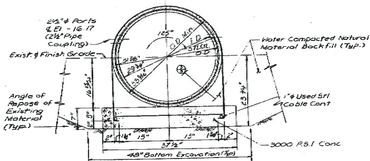
Figure 2. Outfall 001 diffuser cross-section drawing. Source: CDM (1979). "Drawing M-3, Effluent Outfall Diffuser Section Details and Trench Sections".
