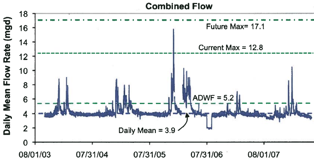
Figure 4. Combined daily mean effluent flow rates for period 10/1/2003 – 5/31/2008, with current daily mean and simulated values indicated.
